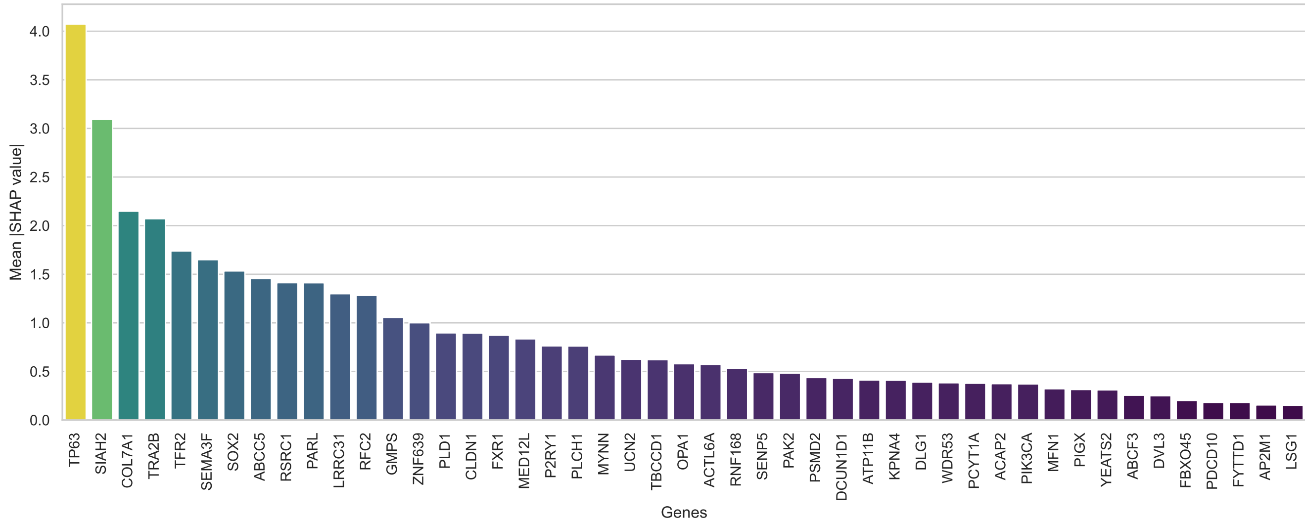
SHAP Analysis of Identified Genes on Combined Data Set
